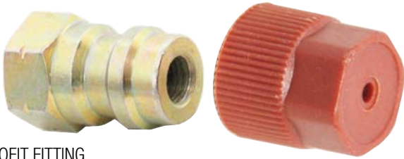
RETROFIT FITTING Baxters Part #: AFA6362 Fitting Size: 3/16" Description: Straight Steel High Side Hose: Fits on to R12 access port Thread: 3/16" Male Flare
